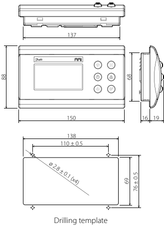
Drilling template
